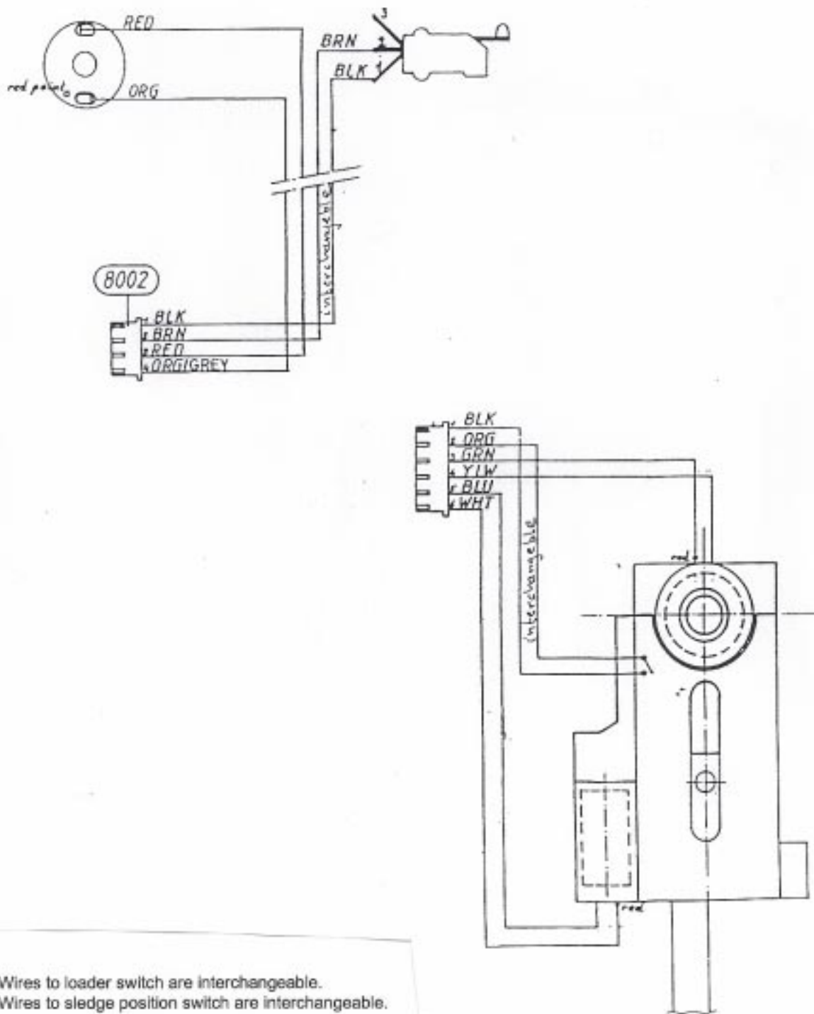
Fig. 3: Recommended wiring diagram
